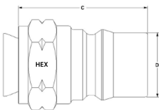
Figure 2 : Plug part
