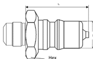
Figure 2: Plug part
