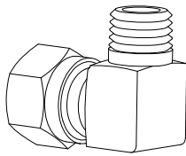
90° Male Elbow (Ref. SAE No. 100202BA)
